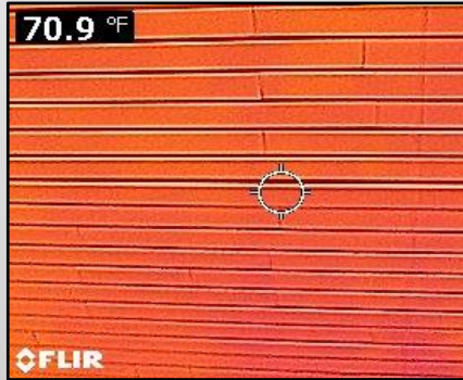
Failed Diffuser
